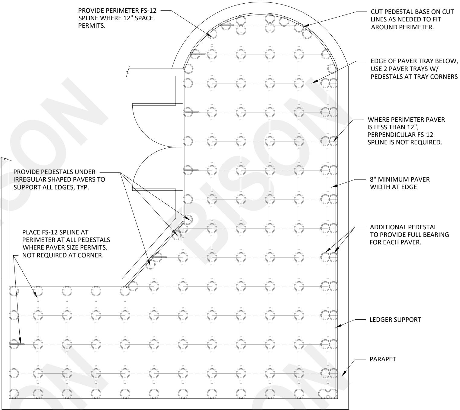
BISON PAVER TRAY/2cm PAVER WIND SYSTEM LAYOUT DIAGRAM 36" TO 48" PAVER LENGTHS - STACK OR RUNNING BOND LAYOUT D8 SCALE: 1/4" = 1'-0"
