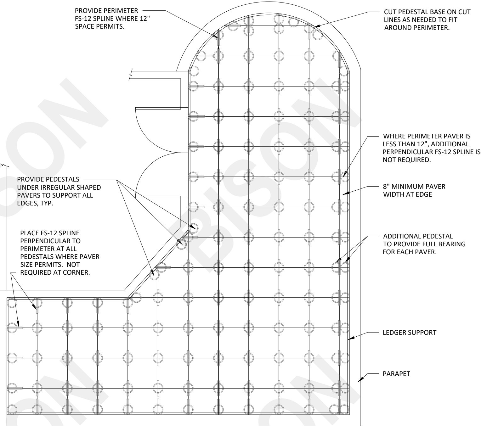
BISON PAVER TRAY/2cm PAVER WIND SYSTEM LAYOUT DIAGRAM 18" TO 24" PAVER LENGTHS - STACK BOND LAYOUT D6 SCALE: 1/4" = 1'-0"
