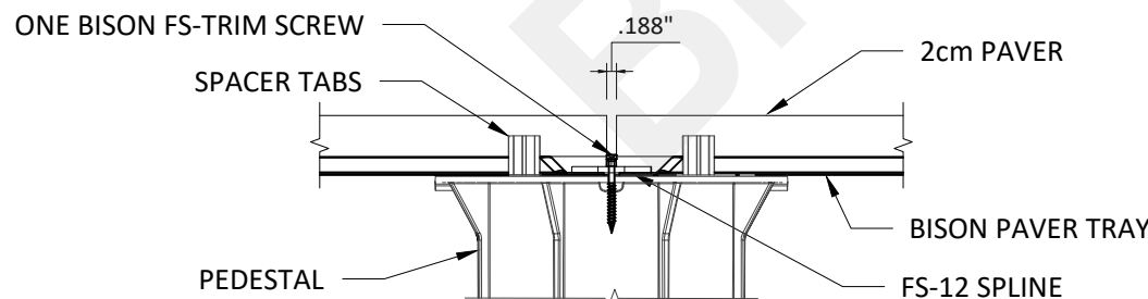
D3 FS-12 SPLINE CONNECTION - SECTION SCALE: 3" = 1'-0"
